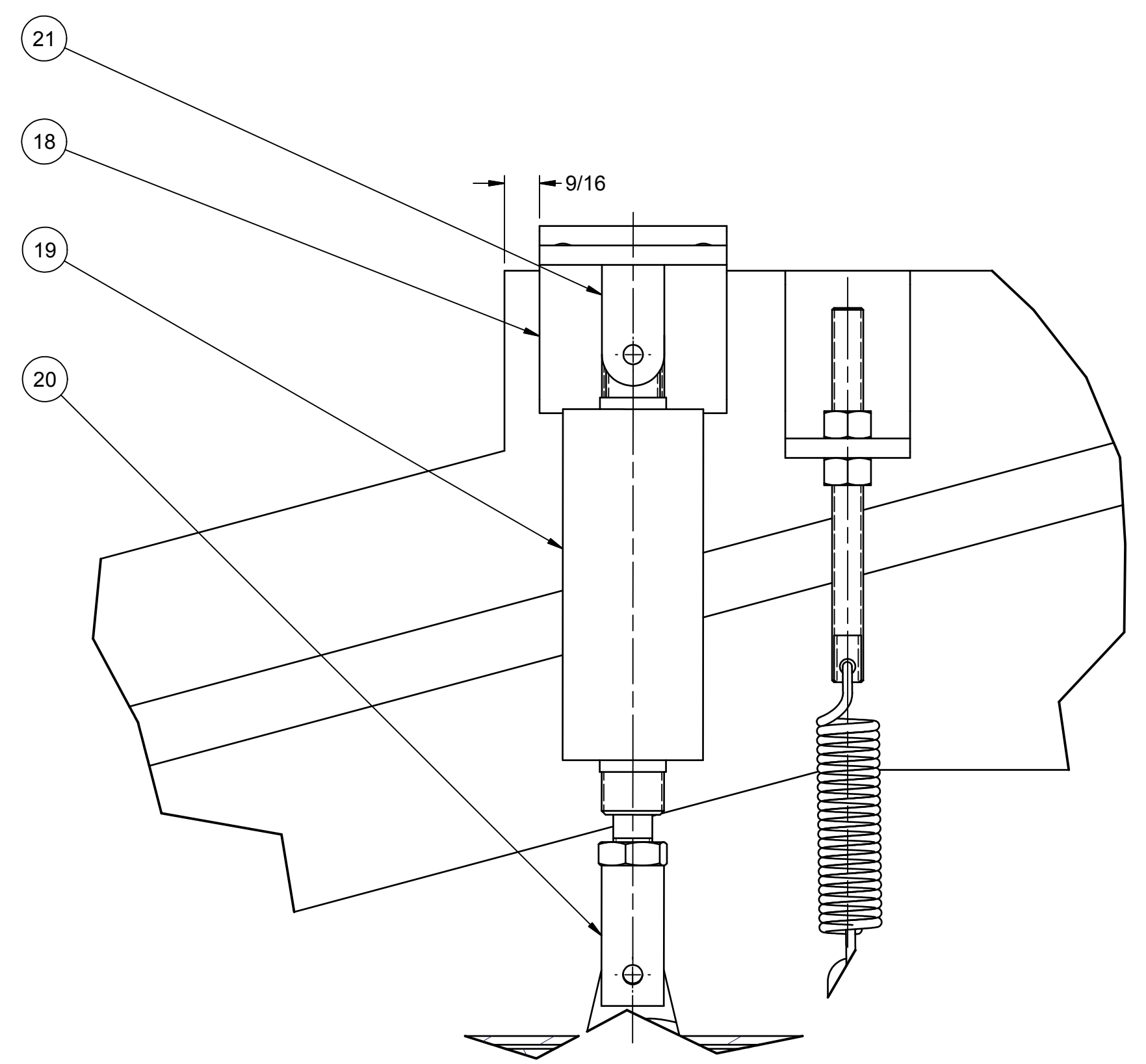
DETAIL B SCALE 1/2 Pneumatic Cylinder Latch Release Option Only
